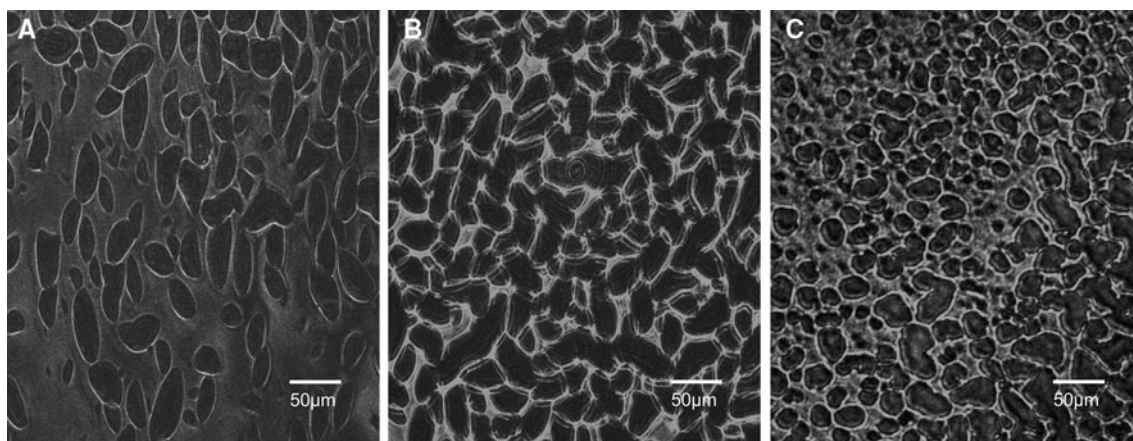
Fig. 2 CLSM micrographs of the genipin-crosslinked gelatin gels at 5 (A), 15 (B) and 25°C (C). The size bar shown represents 50 \mu\text{m}
